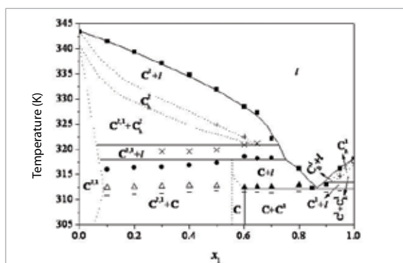
Figure 2. Phase diagram for the system lauric acid (1) + stearic acid (2). (■) fusion temperature; (●) peritectic temperature; (▲) eutectic temperature; (×) metatectic temperature; (+), (Δ), (-) transitions temperatures on the solid phase; (○) transition on the solid phase of the pure component (Costa et al., 2009)
