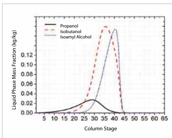
Figure 1. Concentration profiles of high alcohols in bioethanol distillation columns BB1 (Batista and Meirelles, 2009)
