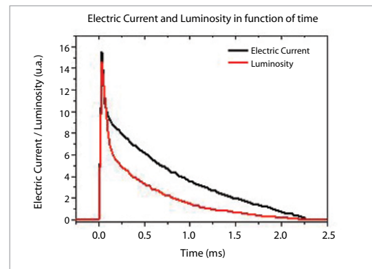
Figure 3. Curves of electric current and luminosity as a function of time
